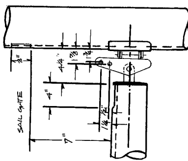
DETAIL 'A' GOOSENECK
