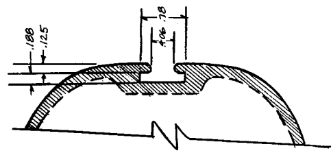
DETAIL 'C' INST. SAIL SLOT
